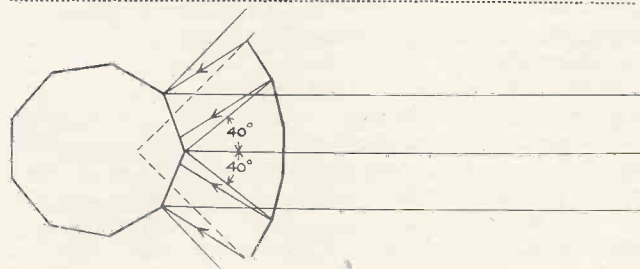
Fig. 8. Light incidence and reflection between ring mirrors and high-speed drum.
