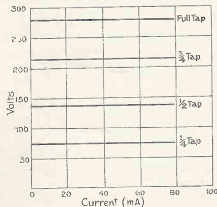
Fig. 3—Typical Stabilovolt characteristics.
