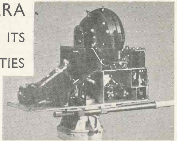
The Marconi-E.M.I. television camera with the case removed.
